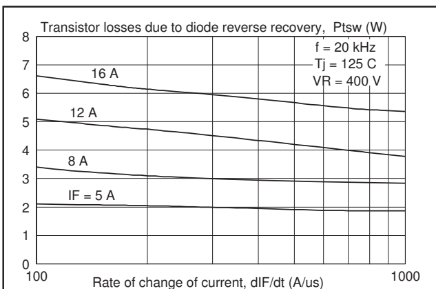
Fig.5. Typical switching losses in transistor due to reverse recovery of diode, as a function of rate of change of current dI_F/dt .
